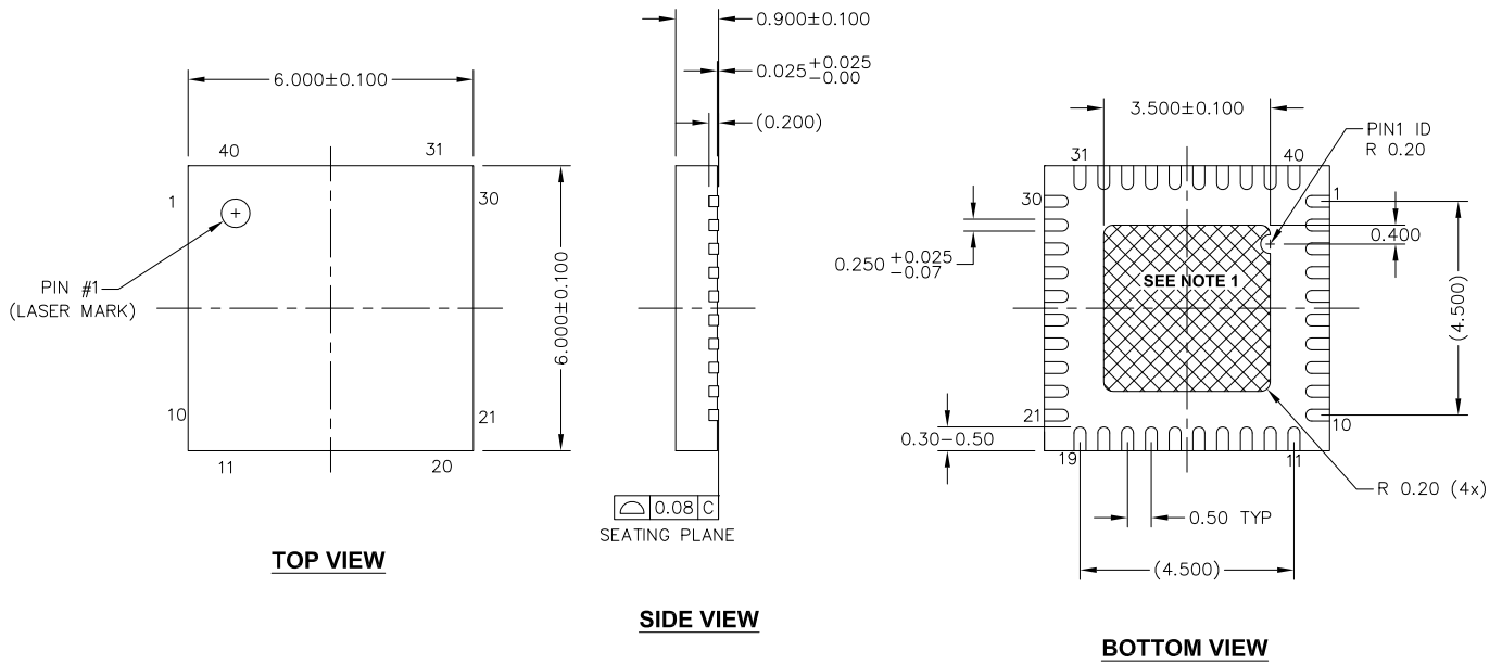
Figure 13. 40-Pin Sawn QFN (6 × 6 × 0.90 mm)
