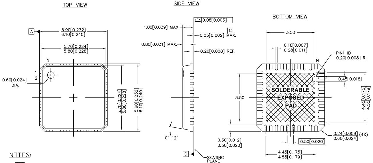
Figure 12. 40-Pin Pb-free QFN 6 x 6 mm
