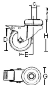
Threaded Stem Castor with Foot Brake
