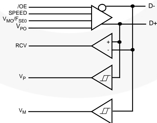
Figure 1. Logic Diagram
