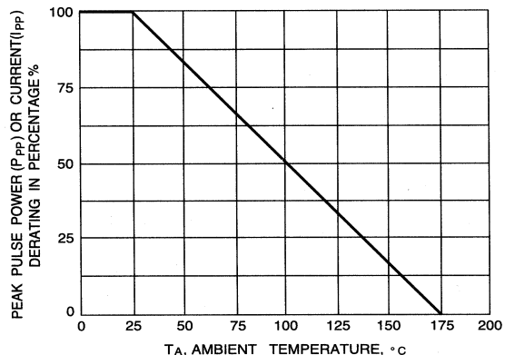
FIGURE 2-PULSE DERATING CURVE
