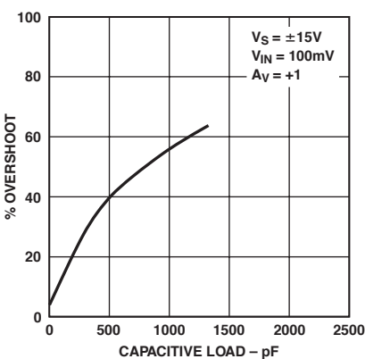
TPC 22. Small-Signal Overshoot vs. Capacitive Load
