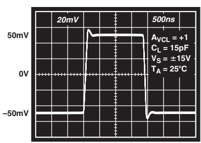
TPC 23. Small-Signal Transient Response
