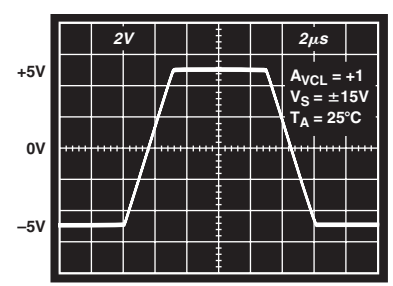
TPC 24. Large-Signal Transient Response
