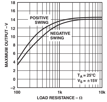
TPC 21. Maximum Output Voltage vs. Load Resistance
