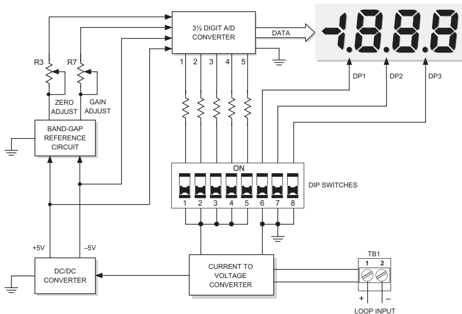
Figure 1. DMS-30LCDA-4/20 Simplified Schematic
