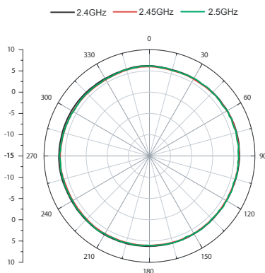
H-Plane Co-Polarization Patterns
