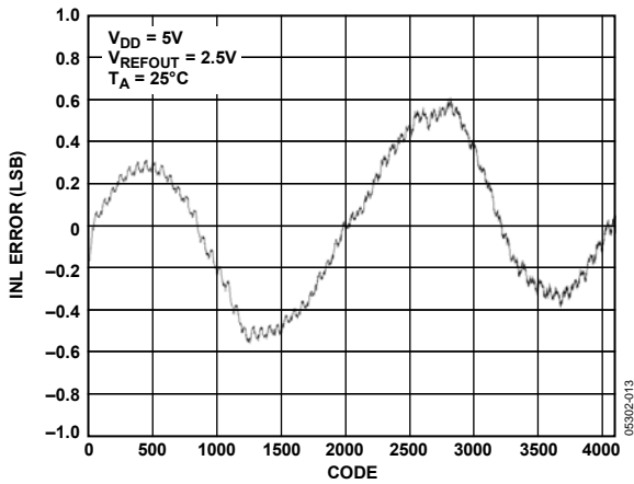
Figure 13. INL AD5628-2
