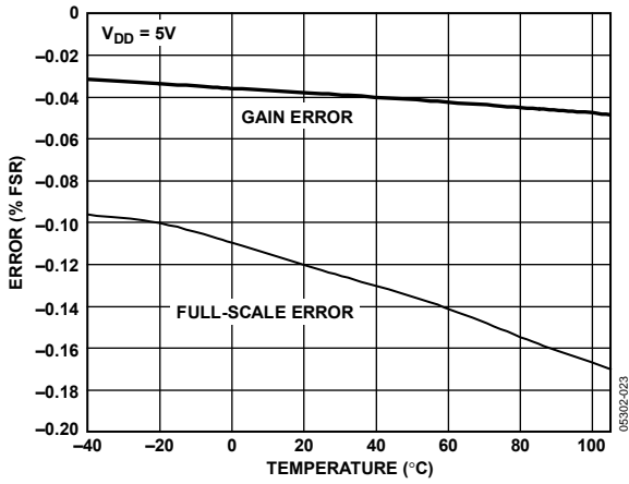
Figure 23. Gain Error and Full-Scale Error vs. Temperature
