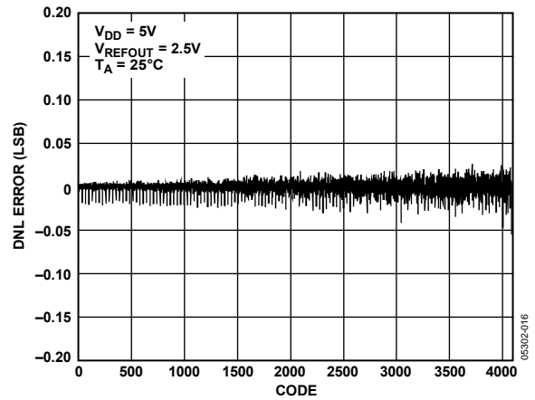
Figure 16. DNL AD5628-2
