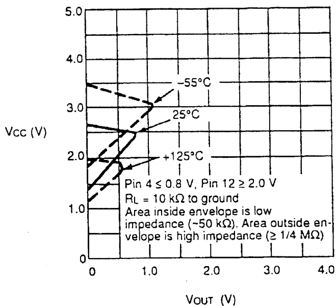
V_{OUT} Versus V_{CC}
