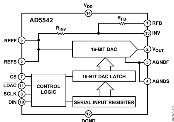
Figure 2. AD5542
