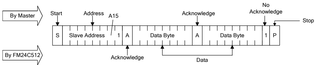
Figure 8. Sequential Read
