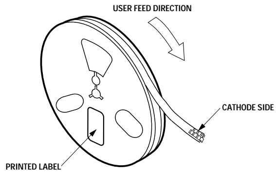
Figure 11. Reeling orientation.
