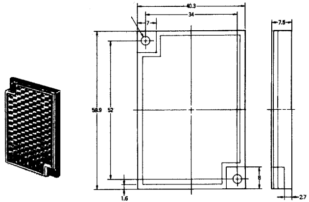
Reflector E39-R1 (Supplied with E32-R16)
