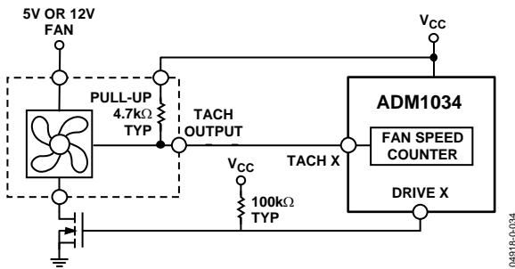
Figure 36. Fan with TACH Pull-Up to +V_{CC}
