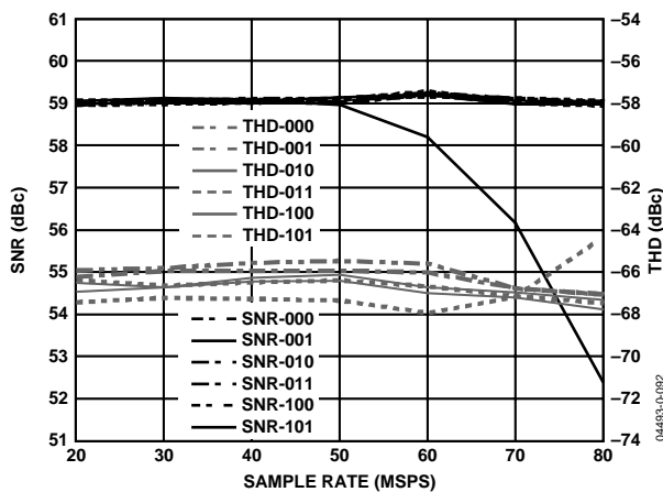
Figure 84. SNR and THD Performance vs. f_{ADC} and SPGA Bias Setting with RxPGA = 0 dB, f_{IN} = 10 MHz, and A_{IN} = -1 dBFS
