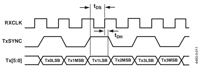
Figure 53. Tx[5:0] Port Full-Duplex Timing Diagram
