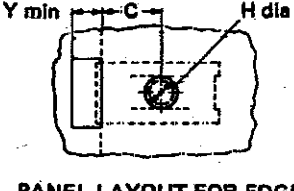
PANEL LAYOUT FOR EDGE OR CENTRE MOUNTING
