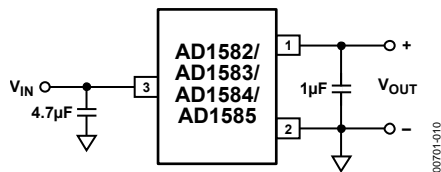
Figure 10. Typical Connection Diagram
