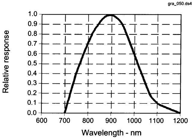
Fig. 5 Spectral Responsivity
