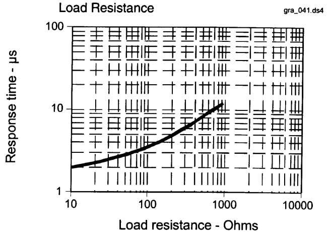
Fig. 4 Non-Saturated Switching Time vs Load Resistance
