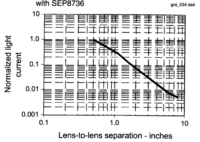
Fig. 6 Coupling Characteristics with SEP8736
