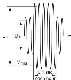
Figure 2. Endurance test
