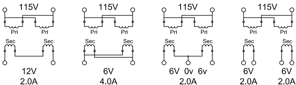
Connection Diagrams for D2044 - 115V supply
