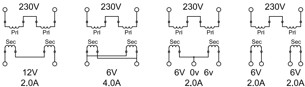
Connection Diagrams for D2044 - 230V supply
