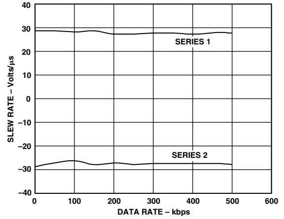
TPC 5. Slew Rate vs. Data Rate
