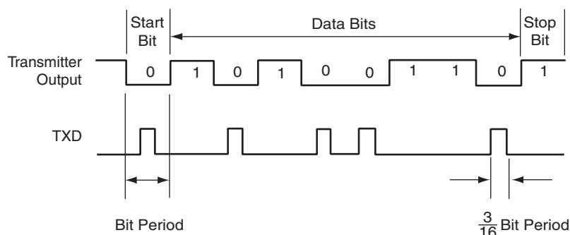
Figure 21-33. IrDA Modulation
