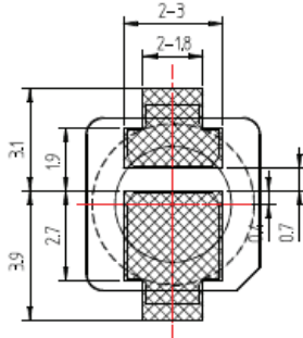
Land Pattern
