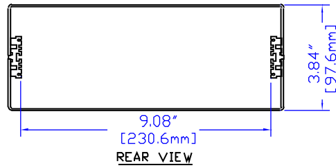
REAR VIEW
