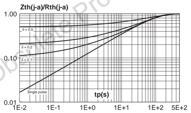
Fig. 4: Variation of thermal impedance to ambient versus pulse duration (recommended pad layout, epoxy FR4, e(\text{Cu}) = 35\mu\text{m} ).
