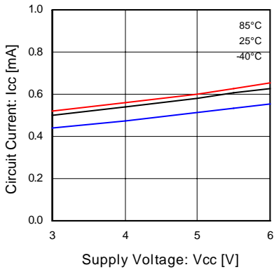
Fig.1 Supply current
