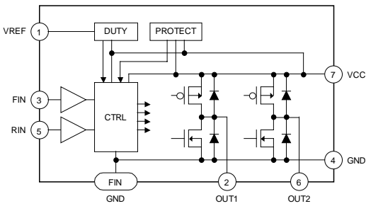
Fig.27 BD6210/11/12HFP
