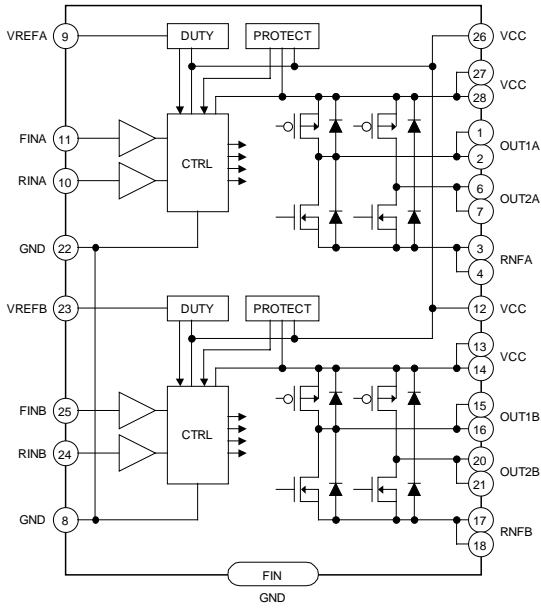
Fig. 36 BD6217FM
