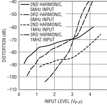
Distortion vs Signal Level V_S = \pm 5V , R_L = 800\Omega at Each Output, T_A = 25^\circ C
