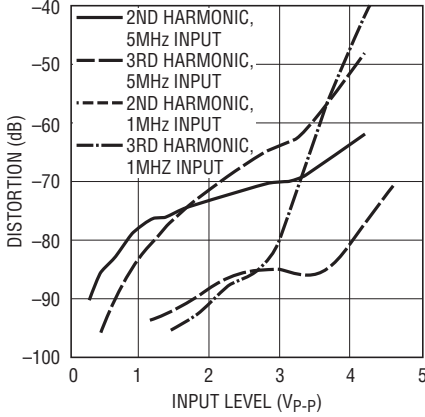
Distortion vs Signal Level V_S = 3V , R_L = 800\Omega at Each Output, T_A = 25^\circ C
