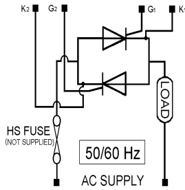
FULL WAVE THYRISTORS
