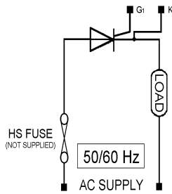
HALF WAVE - THYRISTOR
