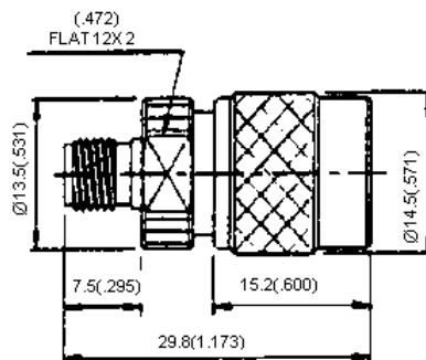
SMA Jack-TNC Plug Part Number: 19-40-1 TGN
