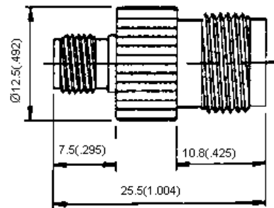
SMA Jack-TNC Jack Part Number: 19-41-4 TGN
