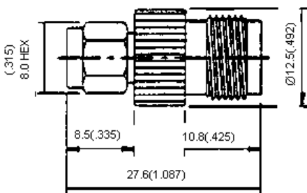
SMA Plug-TNC Jack Part Number: 19-31-3 TGN
