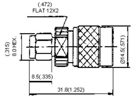
SMA Plug-TNC Plug Part Number: 19-30-1 TGN
