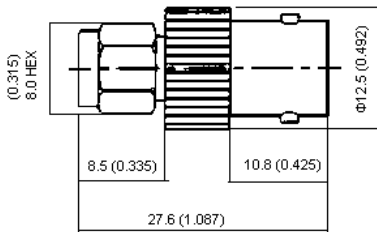
SMA Plug-BNC Jack Part Number: 19-29-1 TGN
