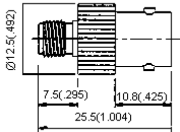
SMA Jack-BNC Jack Part Number: 19-39-4 TGN
