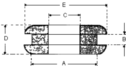
Dimensions: Millimetres
