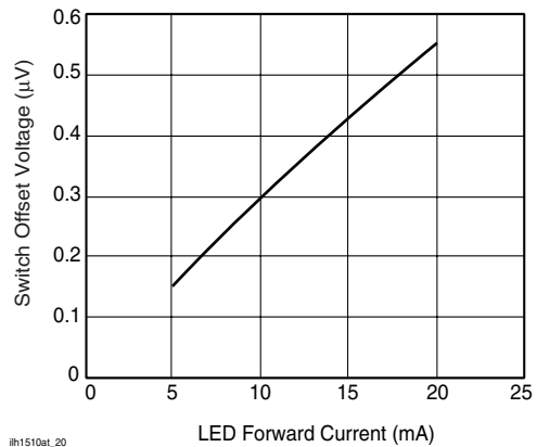
Figure 21. Switch Offset Voltage vs. LED Current
