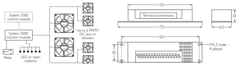
Alarm outputs
