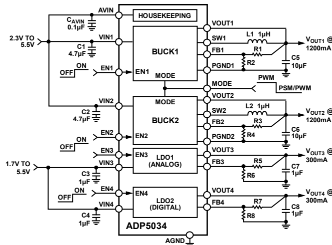
Figure 50. Processor System Power Management with PSM/PWM Control
