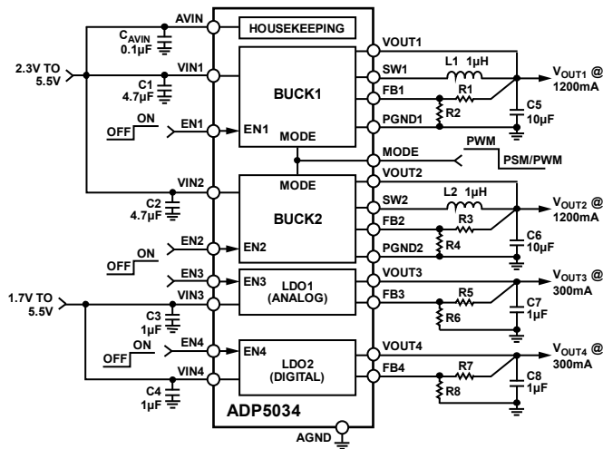
Figure 53. ADP5034 Adjustable Output Voltages with Enable Pins
