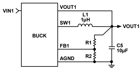
Figure 47. BUCK1 External Output Voltage Setting
