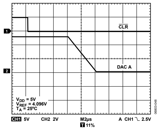
Figure 37. Hardware \overline{\text{CLR}}
