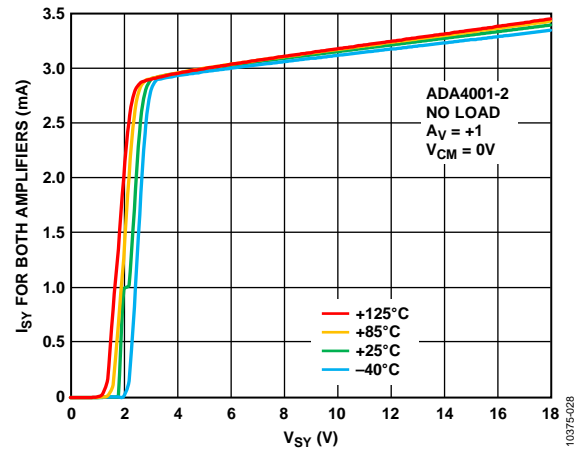
Figure 27. Supply Current vs. Supply Voltage and Temperature
