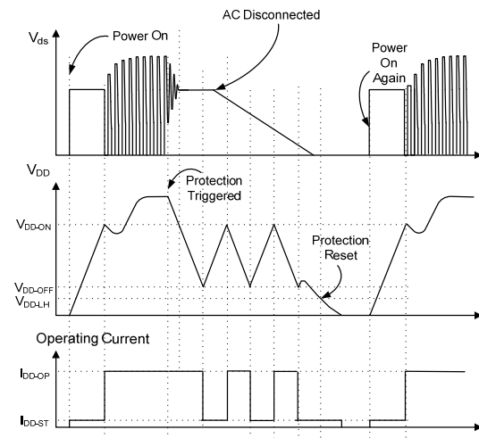
Figure 37. Auto-Restart Mode Operation
