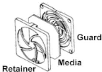
551147 Finger Guard
