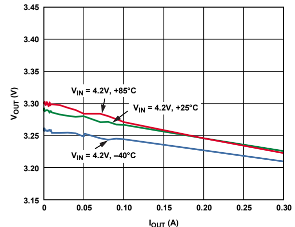
Figure 32. LDO Load Regulation Across Temperature, V_{IN3} = 4.2 V, V_{OUT3} = 3.3 V
