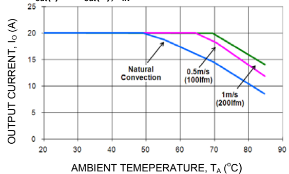
Figure 18. Output Current Derating for the Open Frame Module; Airflow in the Transverse Direction from V_{out(-)} to V_{out(+)} ; V_{IN} = 24V .
