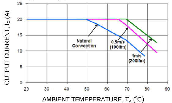
Figure 16. Output Current Derating for the Open Frame Module; Airflow in the Transverse Direction from V_{out(-)} to V_{out(+)} ; V_{IN} = 48V .
