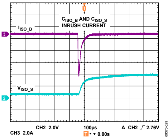
Figure 29. Battery Connect
