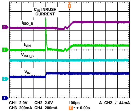
Figure 22. Typical Waveforms, VINx Connect From High Impedance to VBUS, ILIM = 100 mA
