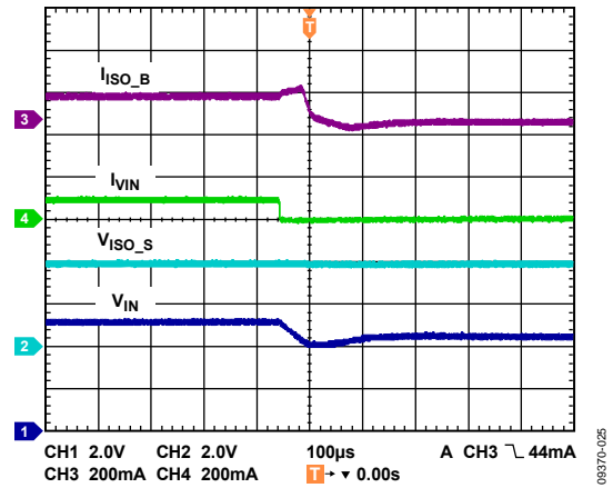
Figure 25. Typical Waveforms, VINx Disconnect from VBUS to High Impedance, ILIM = 100 mA
