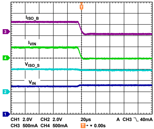
Figure 23. Mode Change, Fast Charge to Suspend (EN_CHG from High to Low), ILIM = 500 mA, R_LOAD = 33 Ω
