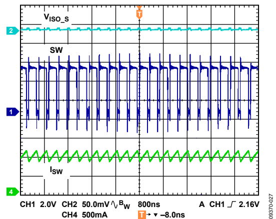
Figure 27. Typical Waveforms, Heavy Load, V_IN = 5.0 V, I_ISO_s = 1000 mA
