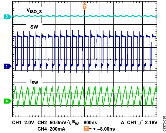
Figure 30. Typical Waveforms, Light Load, V_{IN} = 5.0V , I_{SO,S} = 100mA
