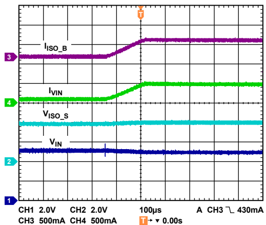
Figure 24. VINx Current Limit Change from 100 mA to 500 mA, EN_CHG = High, V_IN = 5.0 V, R_LOAD = 33 Ω
