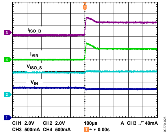
Figure 26. Mode Change, Suspend to Fast Charge (EN_CHG from Low to High), ILIM = 500 mA, R_LOAD = 33 Ω
