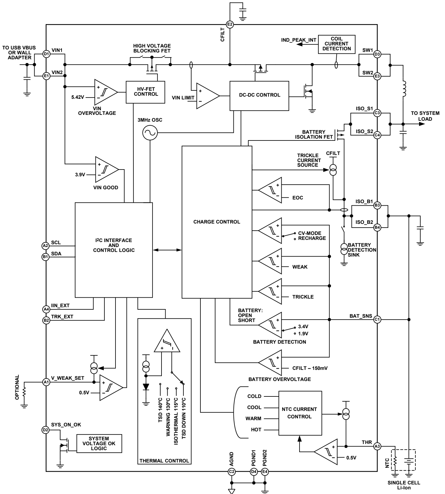
Figure 31. Block Diagram
