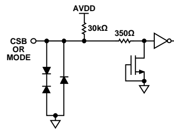
Figure 33. Equivalent CSB and MODE Input Circuit
