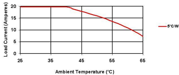
Derating Curve: DC100A20
