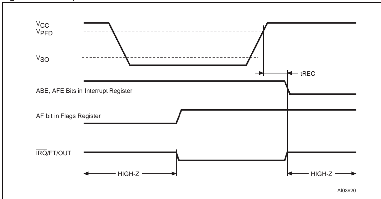
Figure 17. Back-Up Mode Alarm Waveform
