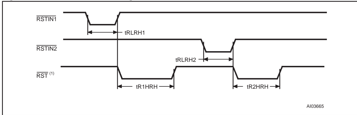
Figure 18. \overline{RSTIN1} & \overline{RSTIN2} Timing Waveforms
