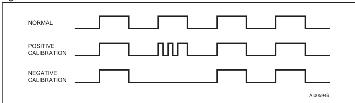
Figure 20. Calibration Waveform
