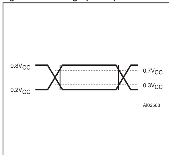
Figure 6. AC Testing Input/Output Waveforms
