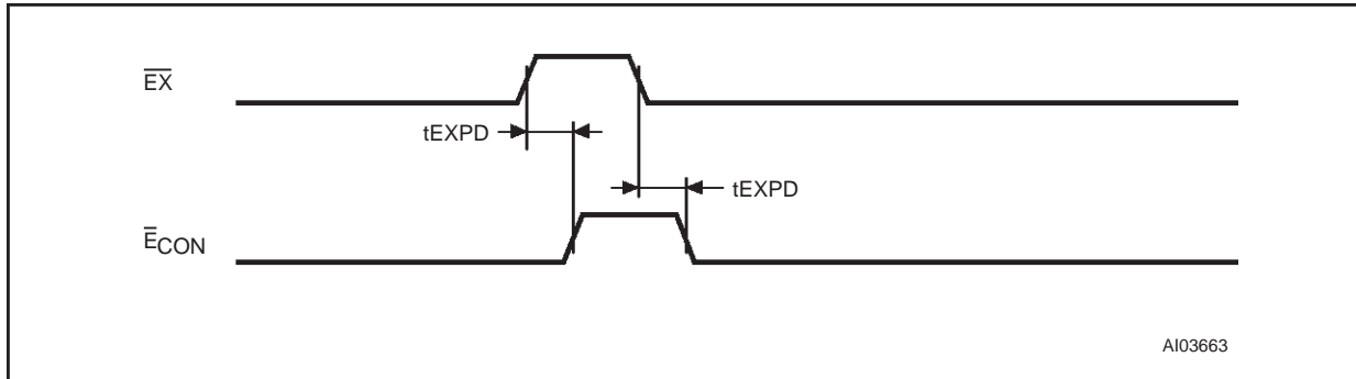
Figure 10. Bus Timing Requirements Sequence
