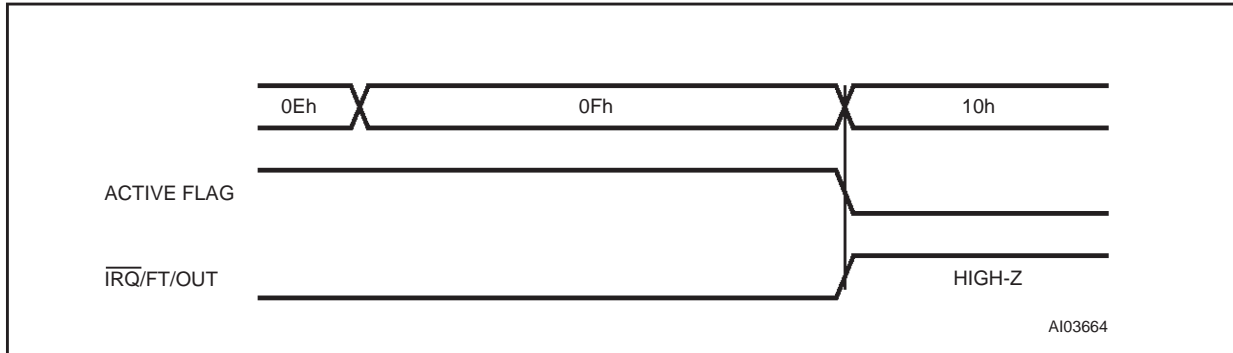
Figure 16. Alarm Interrupt Reset Waveform
