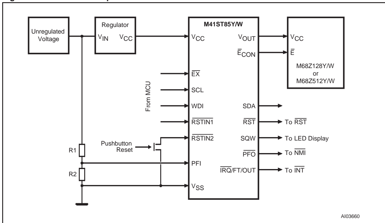
Figure 5. Hardware Hookup
