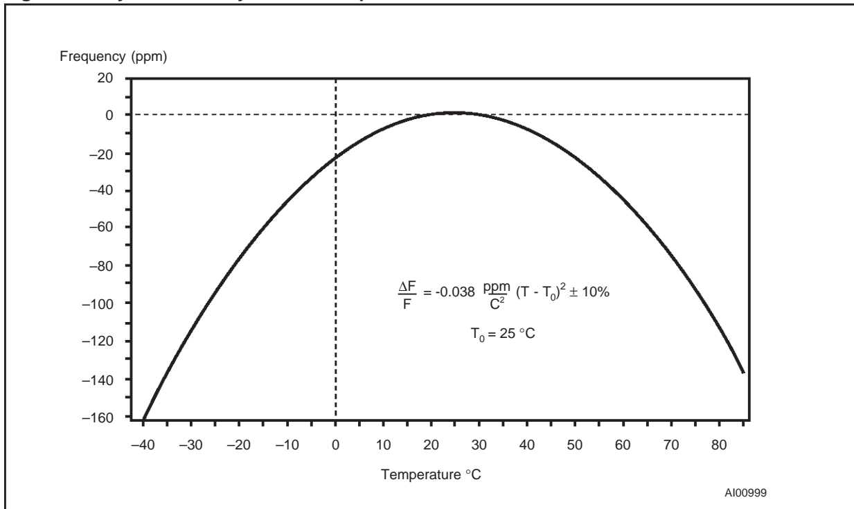
Figure 19. Crystal Accuracy Across Temperature
