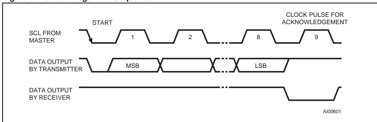
Figure 8. Acknowledgement Sequence
