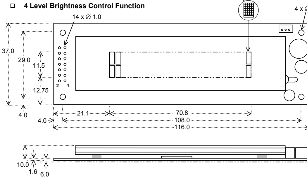
Dimensions in mm See full spec for tolerances
