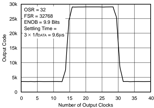
Figure 39. Pulse Response of Sinc 3 Filter ( f_{MOD} = 10MHz )
