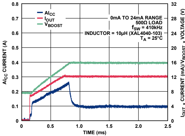
Figure 60. A_{I_{CC}} Current vs. Time for 24 mA Step Through 500 Ω Load with External 51 kΩ Compensation Resistor
