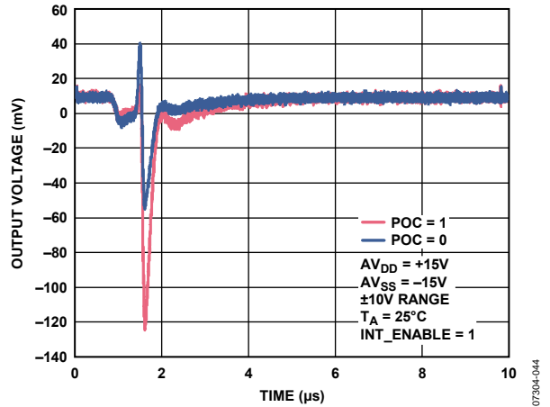
Figure 29. V_{OUT\_x} vs. Time on Output Enable
