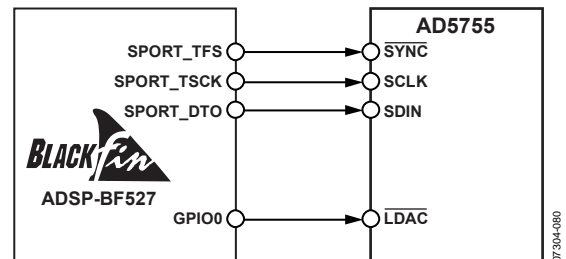
Figure 85. AD5755-to-ADSP-BF527 SPORT Interface
