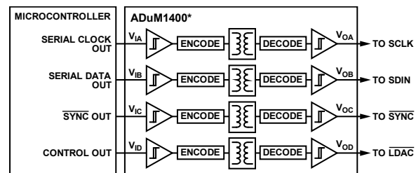
Figure 86. Isolated Interface
