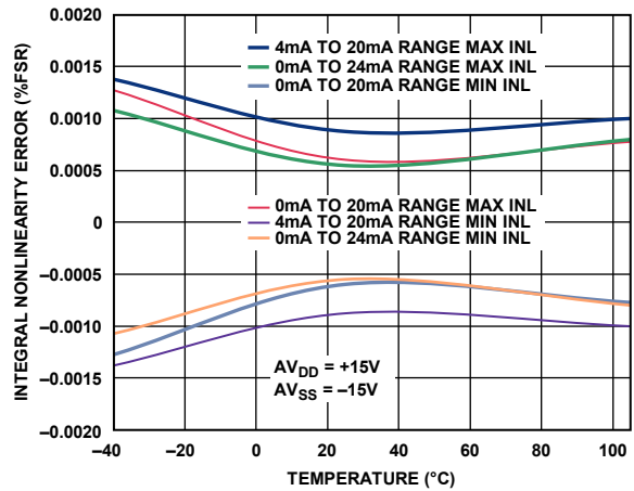
Figure 35. Integral Nonlinearity vs. Temperature, External RSET
