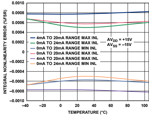
Figure 34. Integral Nonlinearity vs. Temperature, Internal RSET
