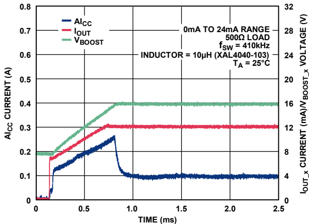
Figure 82. A_{I_{CC}} Current vs. Time for 24 mA Step Through 500 \Omega Load with External 51 k \Omega Compensation Resistor
