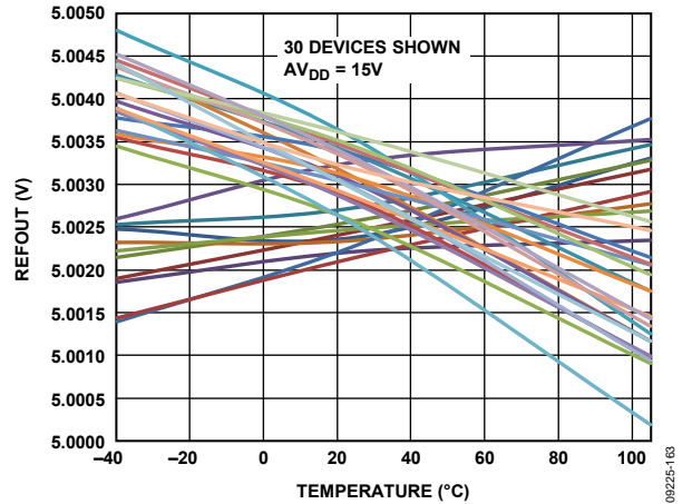
Figure 41. REFOUT vs. Temperature (When the AD5757 is soldered onto a PCB, the reference shifts due to thermal shock on the package. The average output voltage shift is -4\text{ mV} . Measurement of these parts after seven days shows that the outputs typically shift back 2\text{ mV} toward their initial values. This second shift is due to the relaxation of stress incurred during soldering.)
