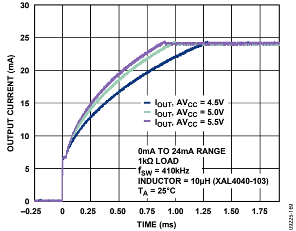
Figure 28. Output Current Settling with DC-to-DC Converter vs. Time and V_{CC} (See Figure 56)
