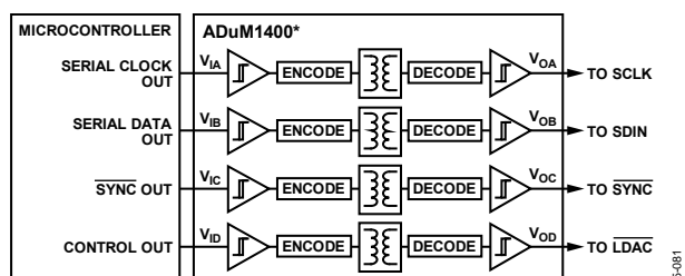
Figure 65. Isolated Interface
