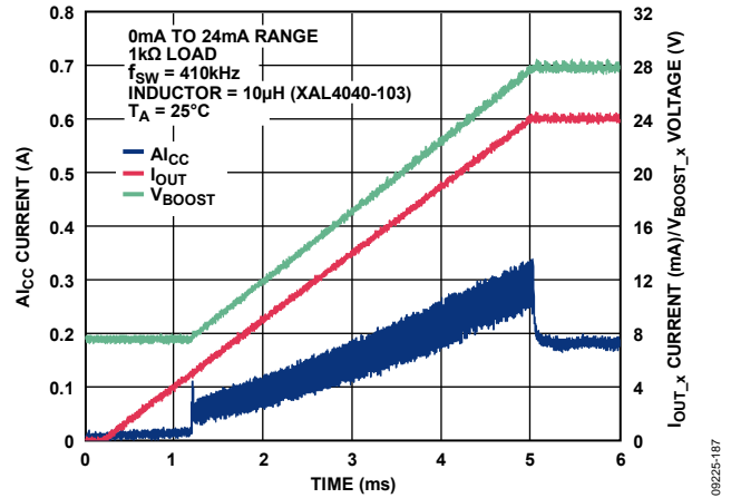
Figure 61. I_{CC} Current vs. Time for 24 mA Slew with Slew Rate Control
