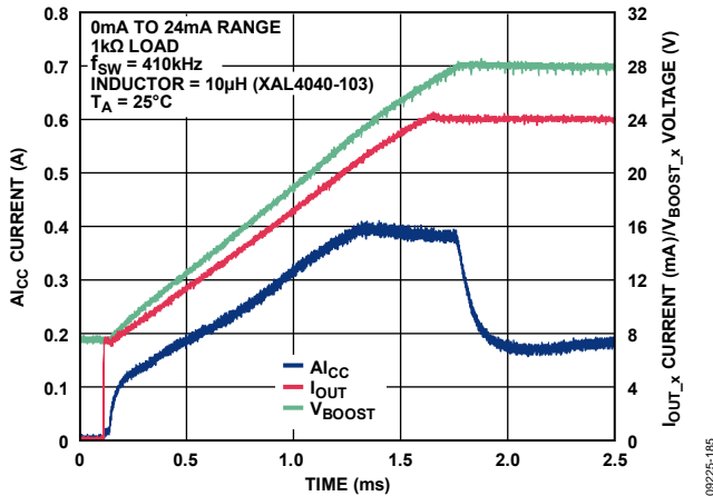
Figure 59. I_{CC} Current vs. Time for 24 mA Through 1 kΩ Slew with External 51 kΩ Compensation Resistor
