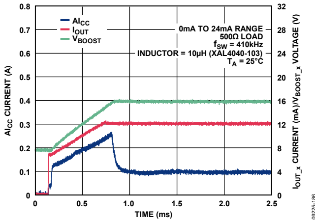
Figure 60. I_{CC} Current vs. Time for 24 mA Through 500 Ω Slew with External 51 kΩ Compensation Resistor
