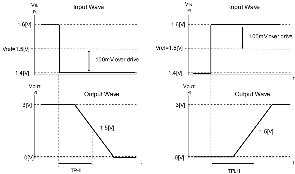
Fig4. Slew rate
