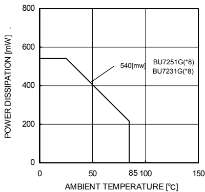
Fig6. Thermal resistance and power dissipation
