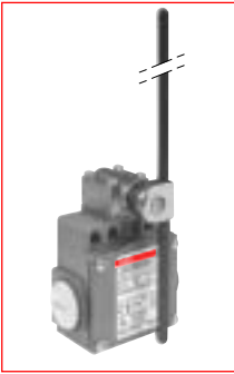
Adjustable ø6 polyamide rod lever
